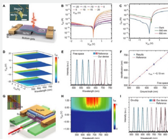
Figure 3. Narrow-band spectral sensing.
