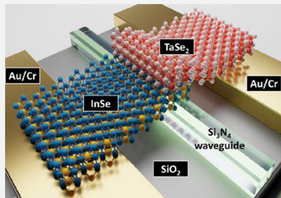
Figure 1: 3D schematic diagram of InSe/TaSe 2 heterostructure transferred on top of a Si 3 N 4 waveguide and pre-patterned Au/Cr metal contacts.
