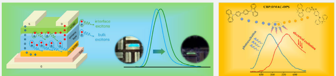
Figure 4. Tunability of emission in organic light-emitting transistor by (left): interface engineering and (right) electric field.
